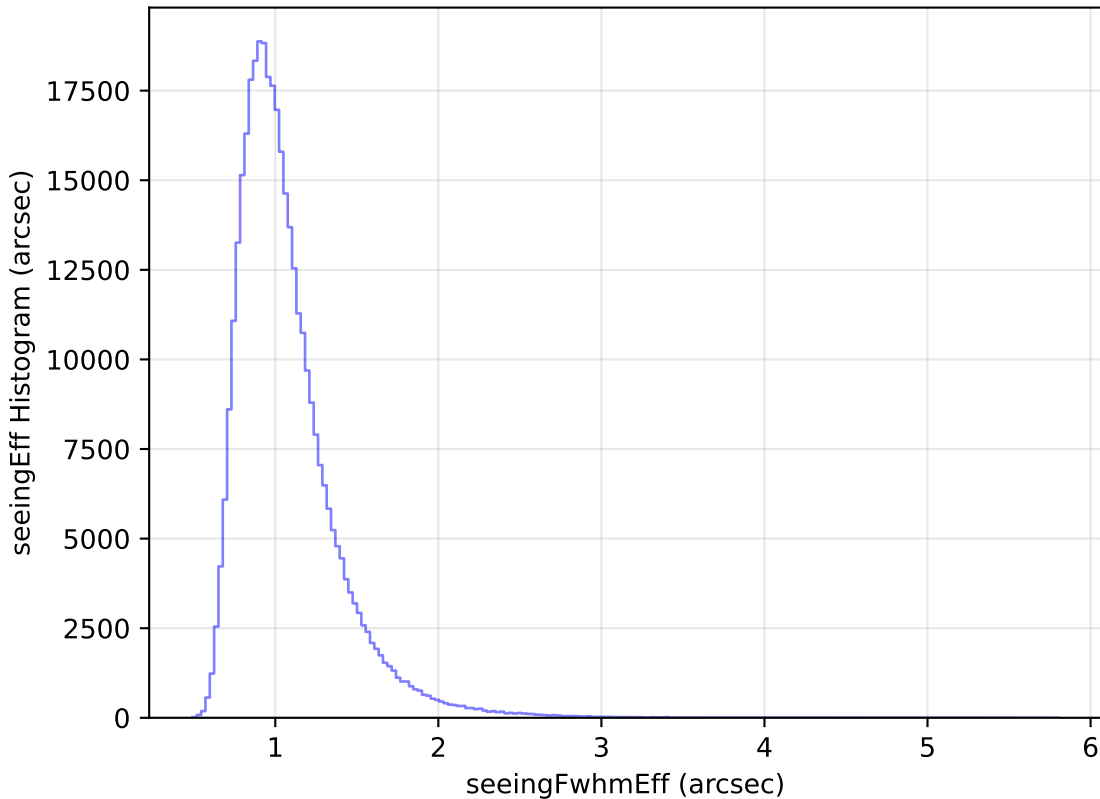
roman_v3.3_10yrs All sky y band: seeingEff Histogram
