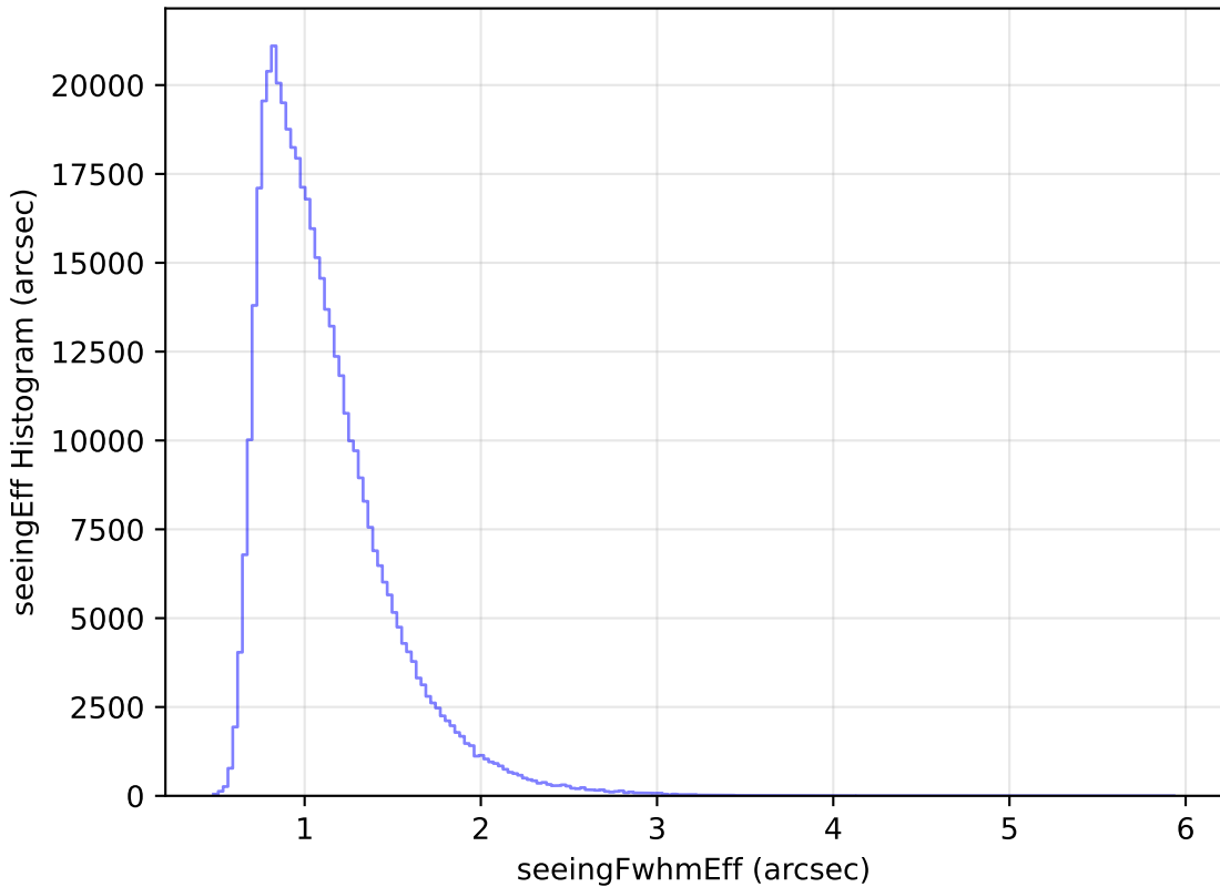
roman_v3.3_10yrs All sky r band: seeingEff Histogram
