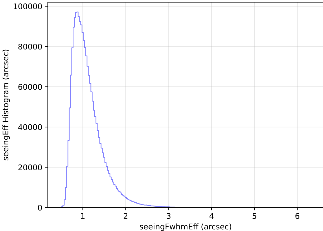
roman_v3.3_10yrs All sky all bands: seeingEff Histogram
