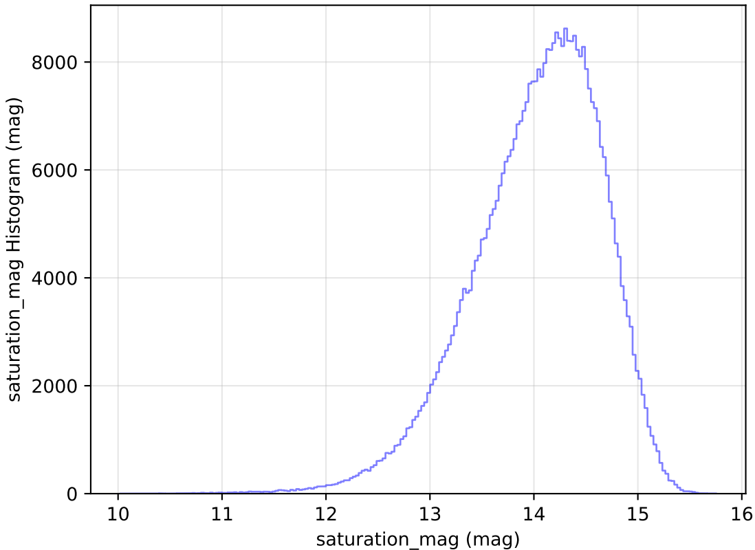
roman_v3.3_10yrs WFD z band: saturation_mag Histogram
