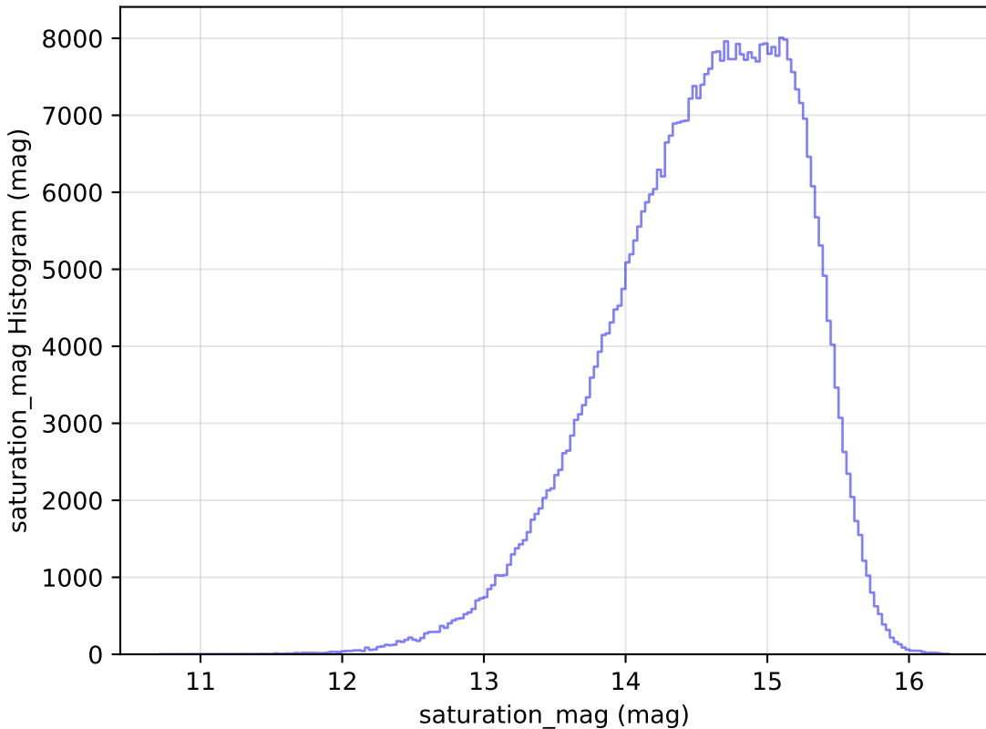
roman_v3.3_10yrs WFD r band: saturation_mag Histogram
