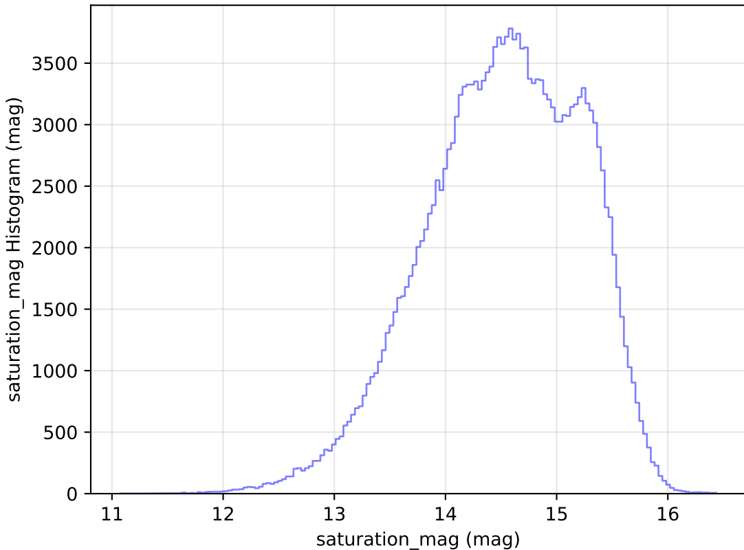
roman_v3.3_10yrs WFD g band: saturation_mag Histogram
