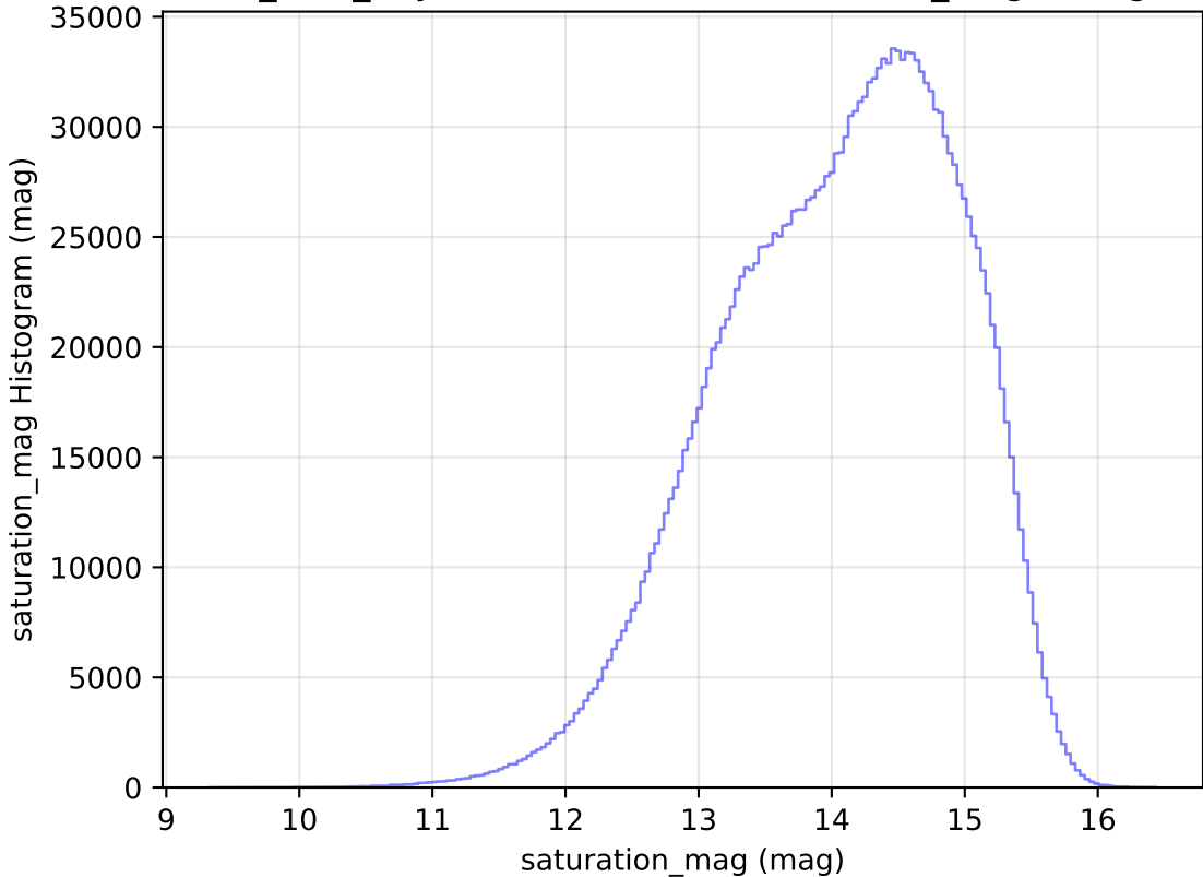
roman_v3.3_10yrs WFD all bands: saturation_mag Histogram
