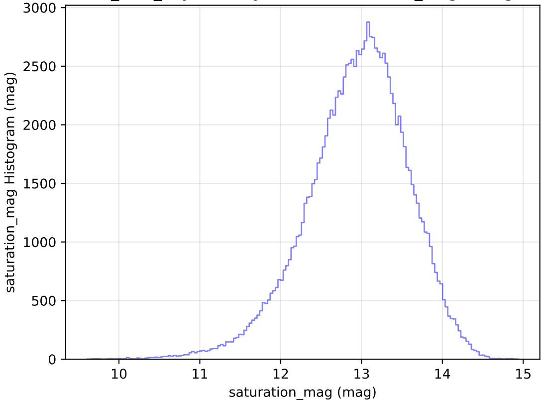
roman_v3.3_10yrs All sky u band: saturation_mag Histogram
