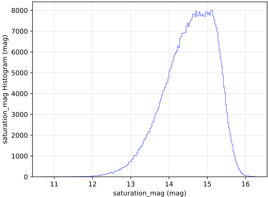
roman_v3.3_10yrs All sky r band: saturation_mag Histogram
