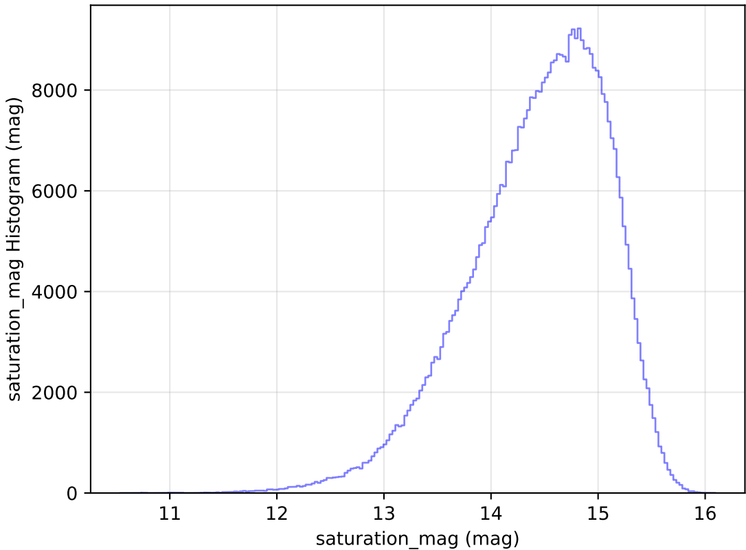
roman_v3.3_10yrs All sky i band: saturation_mag Histogram
