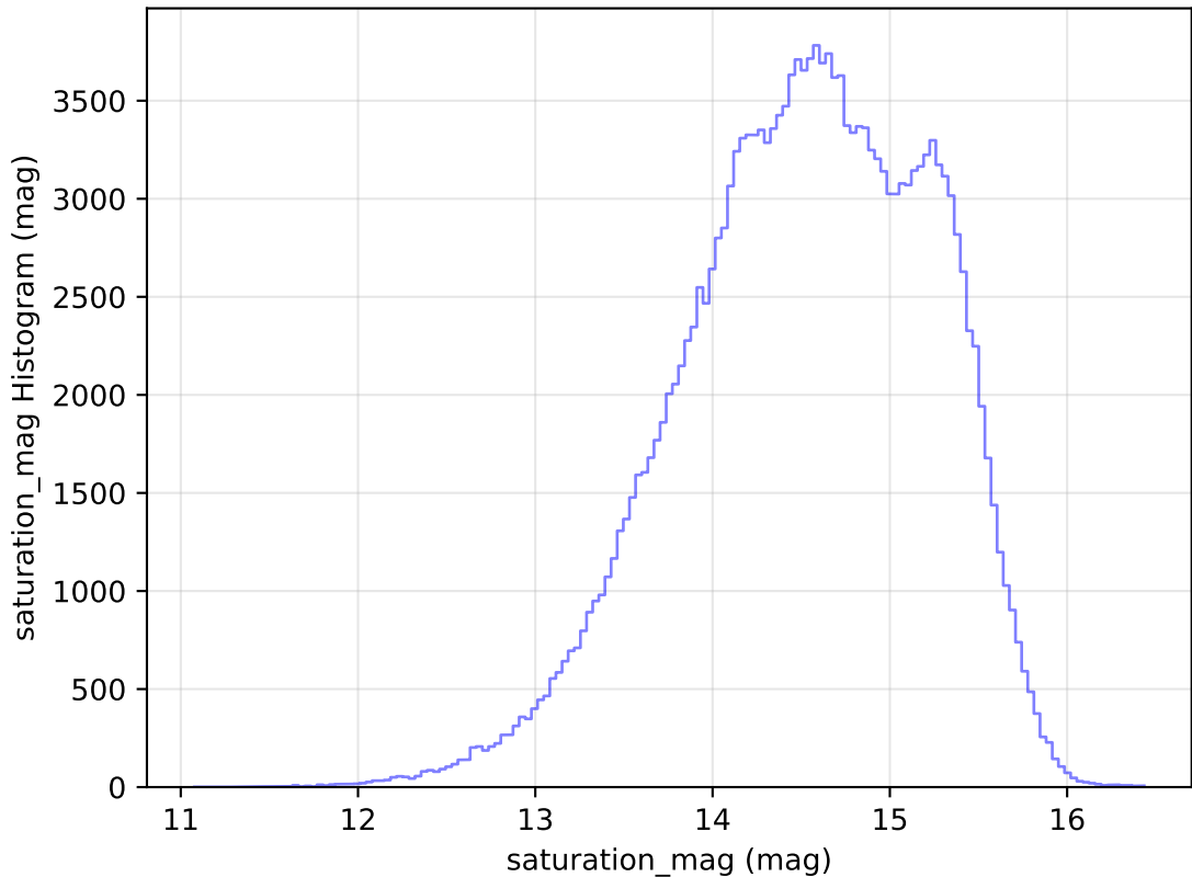
roman_v3.3_10yrs All sky g band: saturation_mag Histogram
