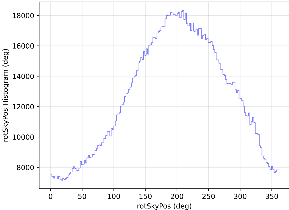
roman_v3.3_10yrs WFD all bands: rotSkyPos Histogram
