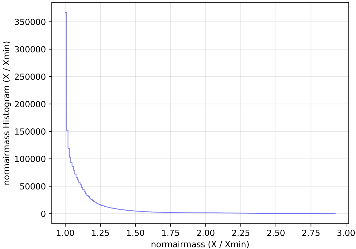
roman_v3.3_10yrs WFD all bands: normairmass Histogram
