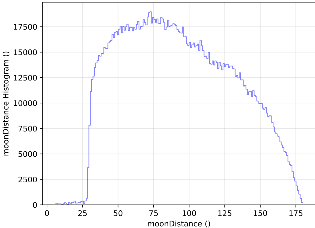
roman_v3.3_10yrs WFD all bands: moonDistance Histogram
