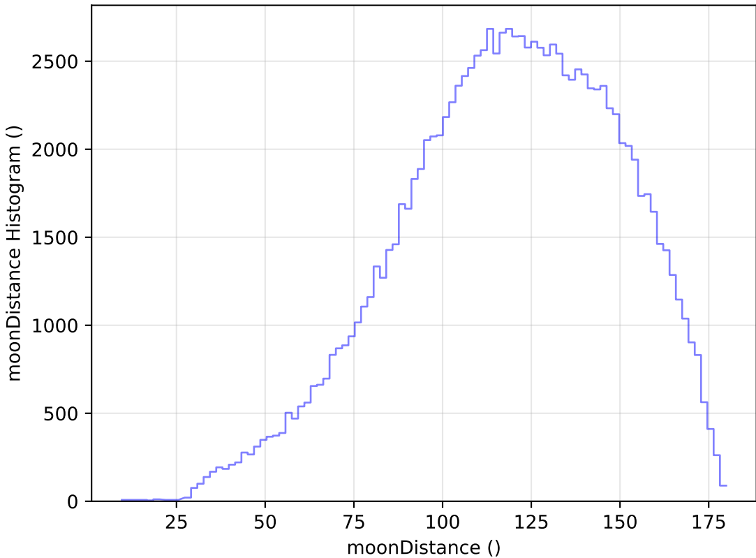
roman_v3.3_10yrs All sky u band: moonDistance Histogram
