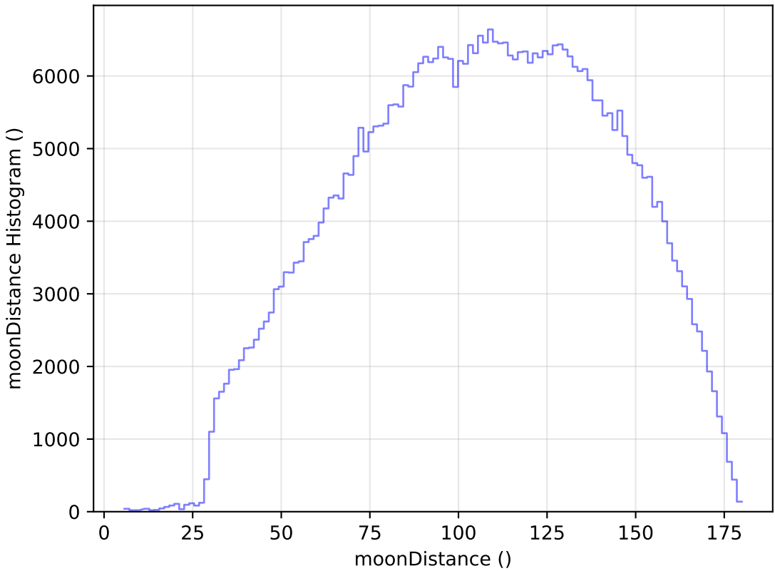
roman_v3.3_10yrs All sky r band: moonDistance Histogram
