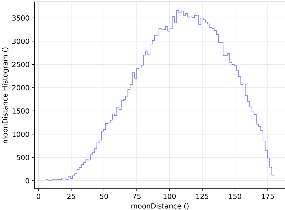
roman_v3.3_10yrs All sky g band: moonDistance Histogram
