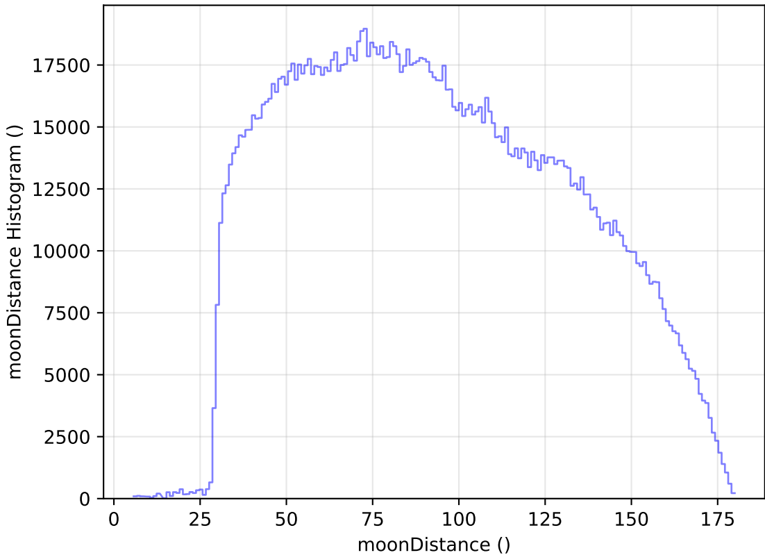
roman_v3.3_10yrs All sky all bands: moonDistance Histogram
