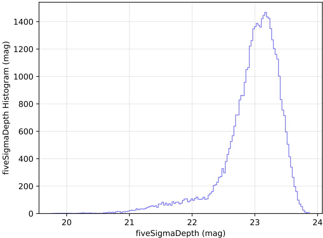
roman_v3.3_10yrs Yr 1 z band: fiveSigmaDepth Histogram
