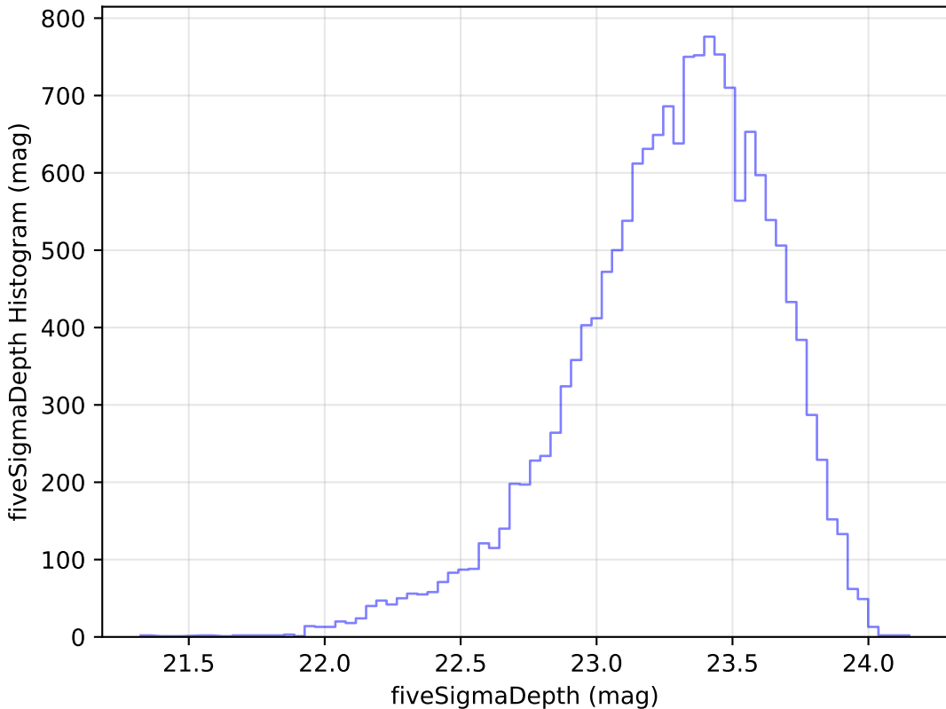
roman_v3.3_10yrs Yr 1 u band: fiveSigmaDepth Histogram
