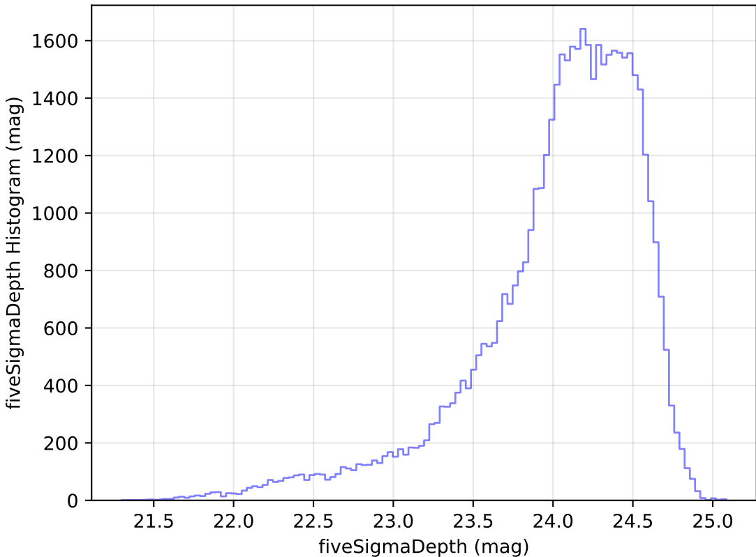
roman_v3.3_10yrs Yr 1 r band: fiveSigmaDepth Histogram
