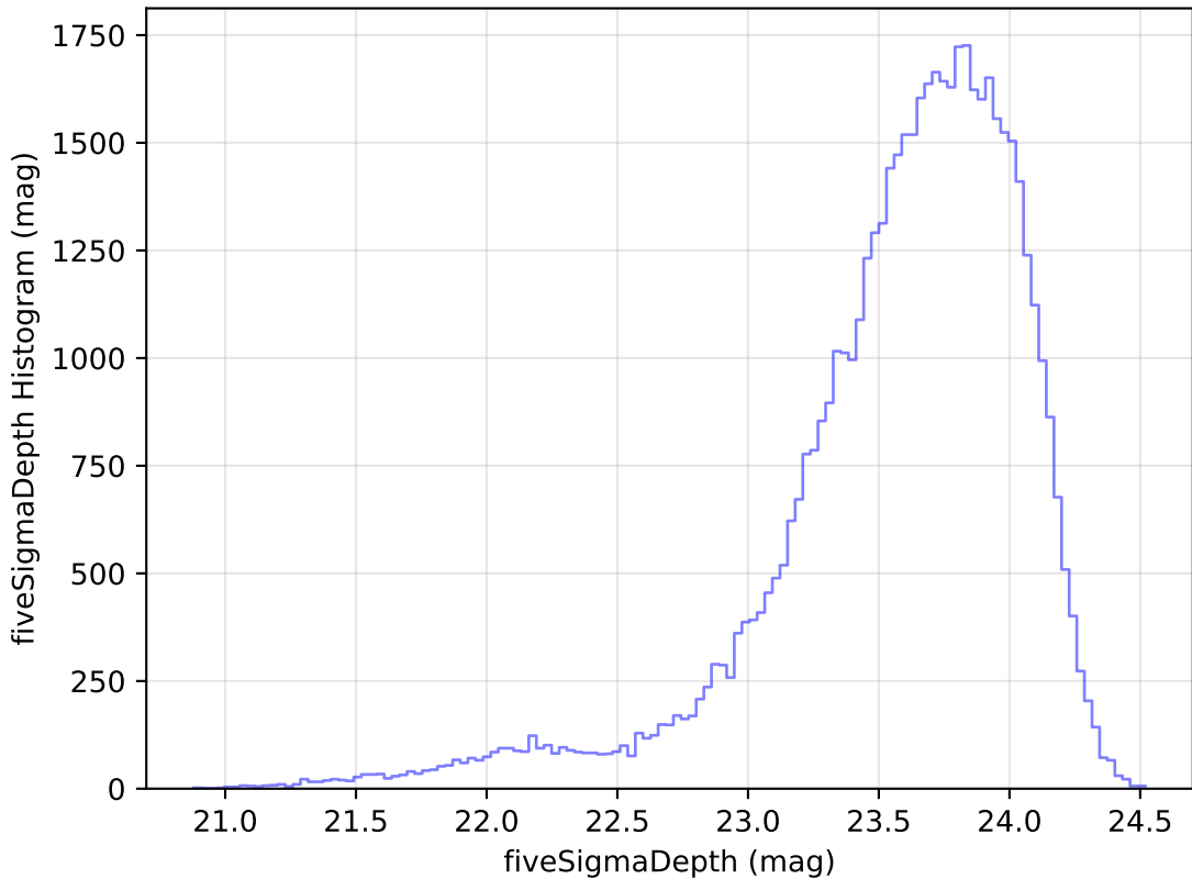
roman_v3.3_10yrs Yr 1 i band: fiveSigmaDepth Histogram
