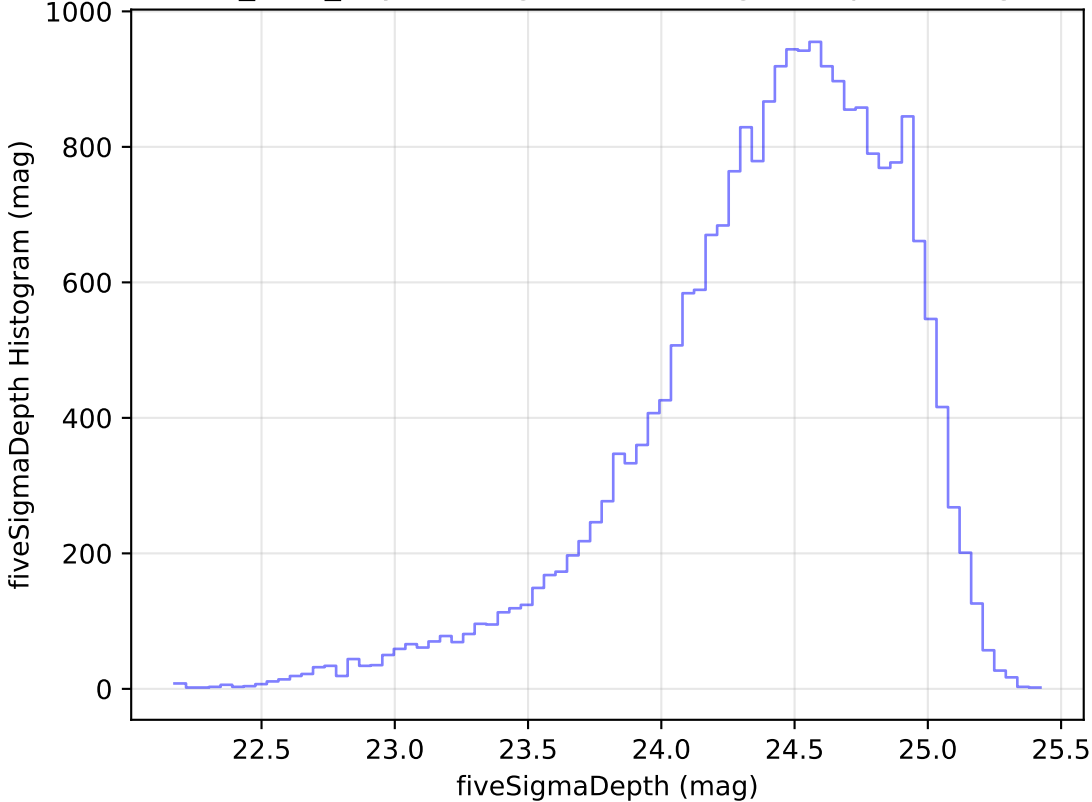
roman_v3.3_10yrs Yr 1 g band: fiveSigmaDepth Histogram
