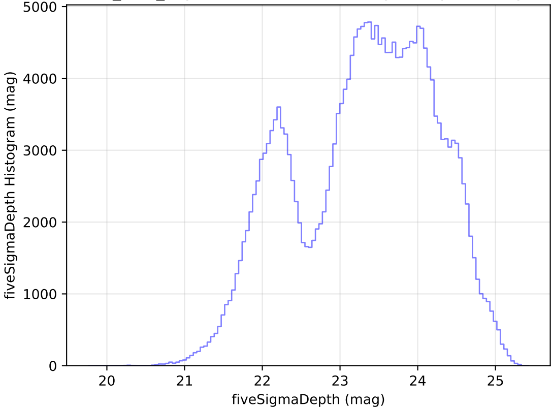
roman_v3.3_10yrs Yr 1 all bands: fiveSigmaDepth Histogram
