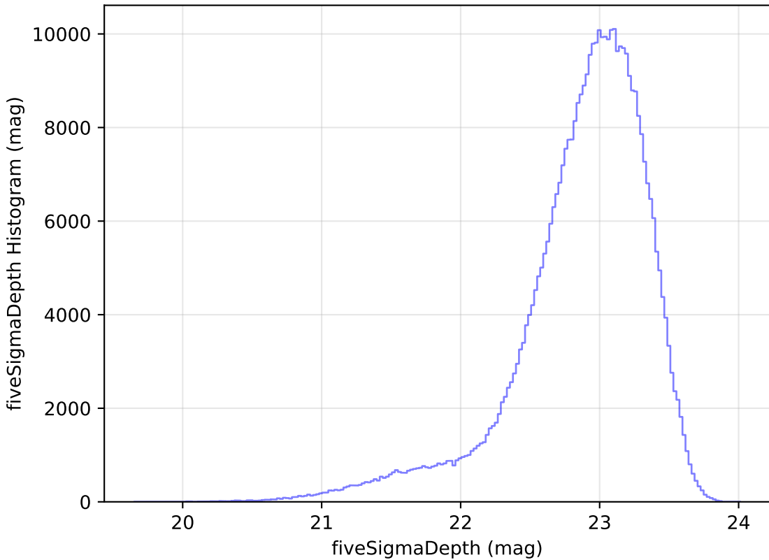
roman_v3.3_10yrs WFD z band: fiveSigmaDepth Histogram
