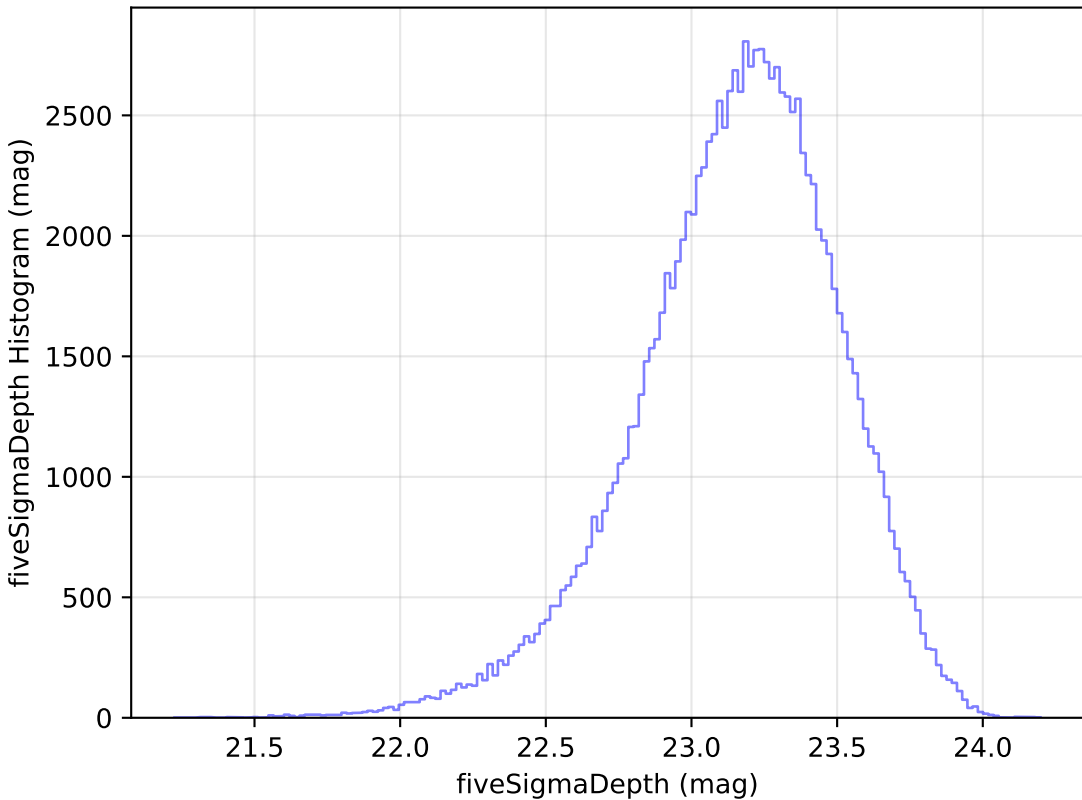
roman_v3.3_10yrs WFD u band: fiveSigmaDepth Histogram
