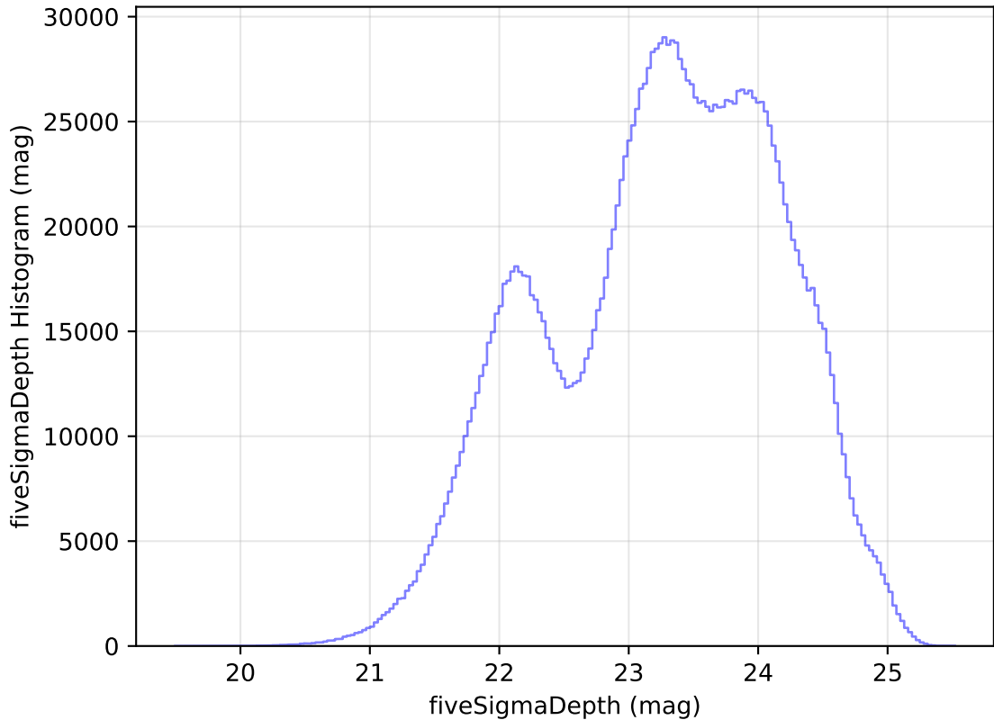
roman_v3.3_10yrs WFD all bands: fiveSigmaDepth Histogram
