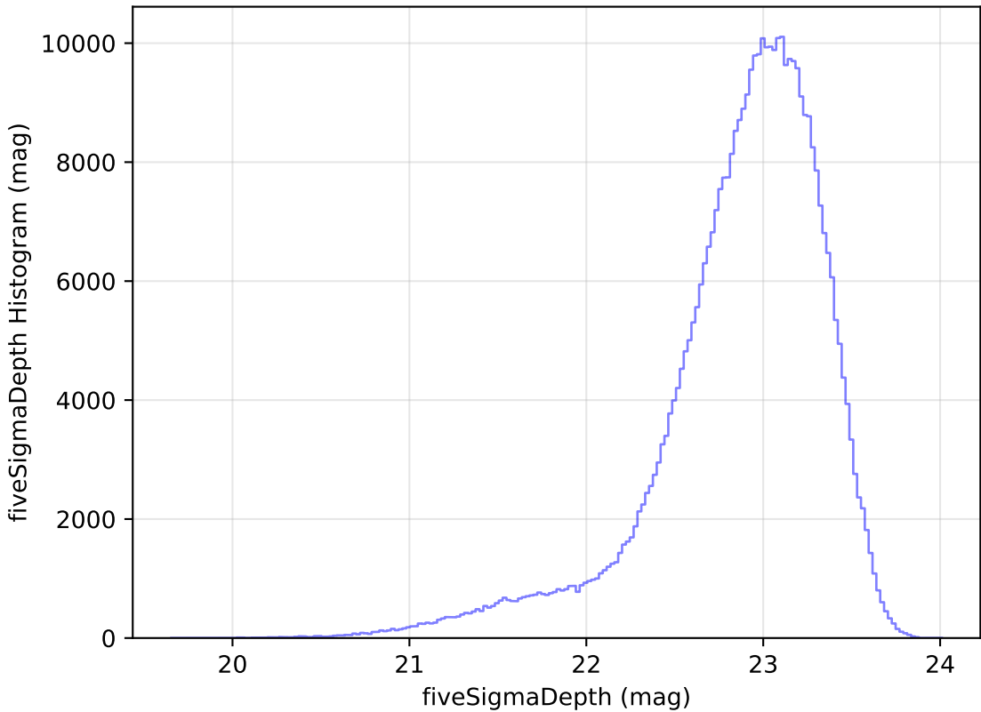
roman_v3.3_10yrs All sky z band: fiveSigmaDepth Histogram
