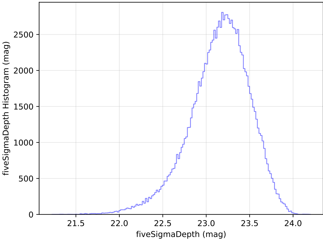
roman_v3.3_10yrs All sky u band: fiveSigmaDepth Histogram
