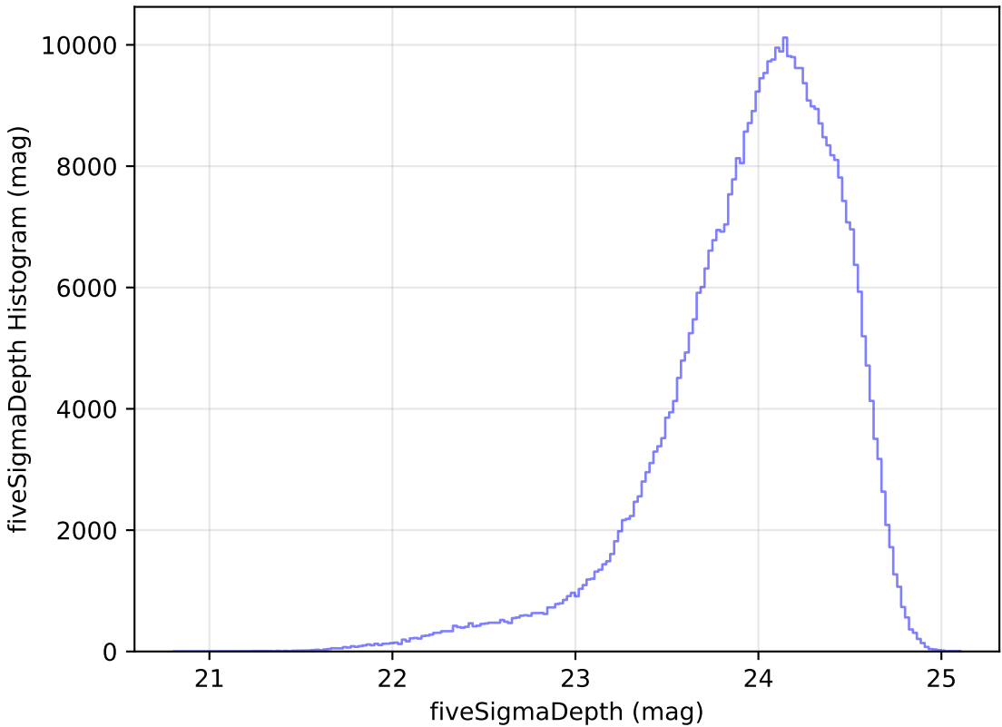
roman_v3.3_10yrs All sky r band: fiveSigmaDepth Histogram
