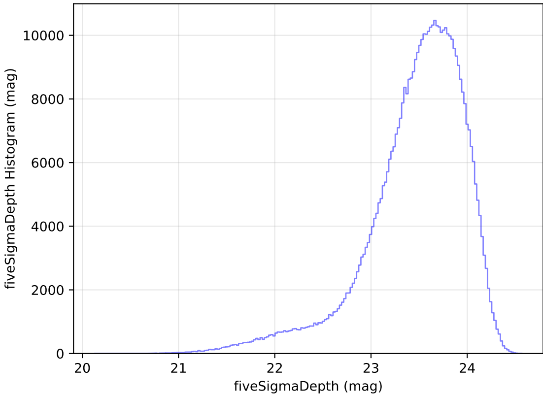
roman_v3.3_10yrs All sky i band: fiveSigmaDepth Histogram
