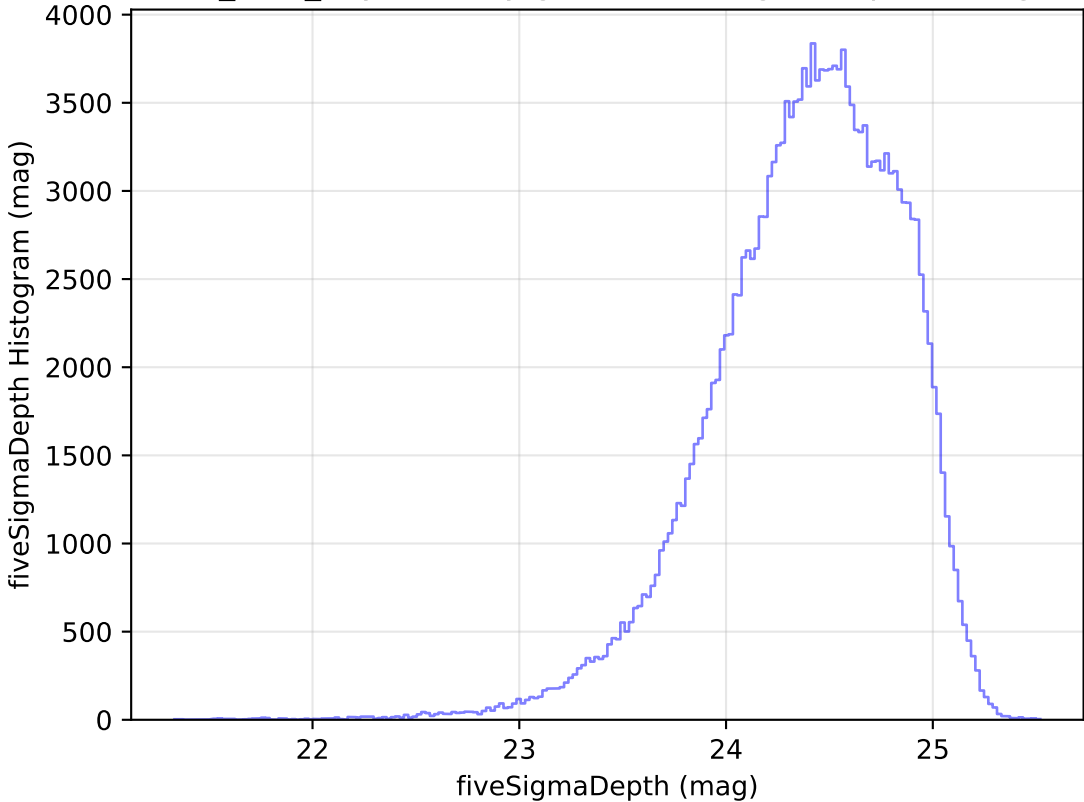
roman_v3.3_10yrs All sky g band: fiveSigmaDepth Histogram
