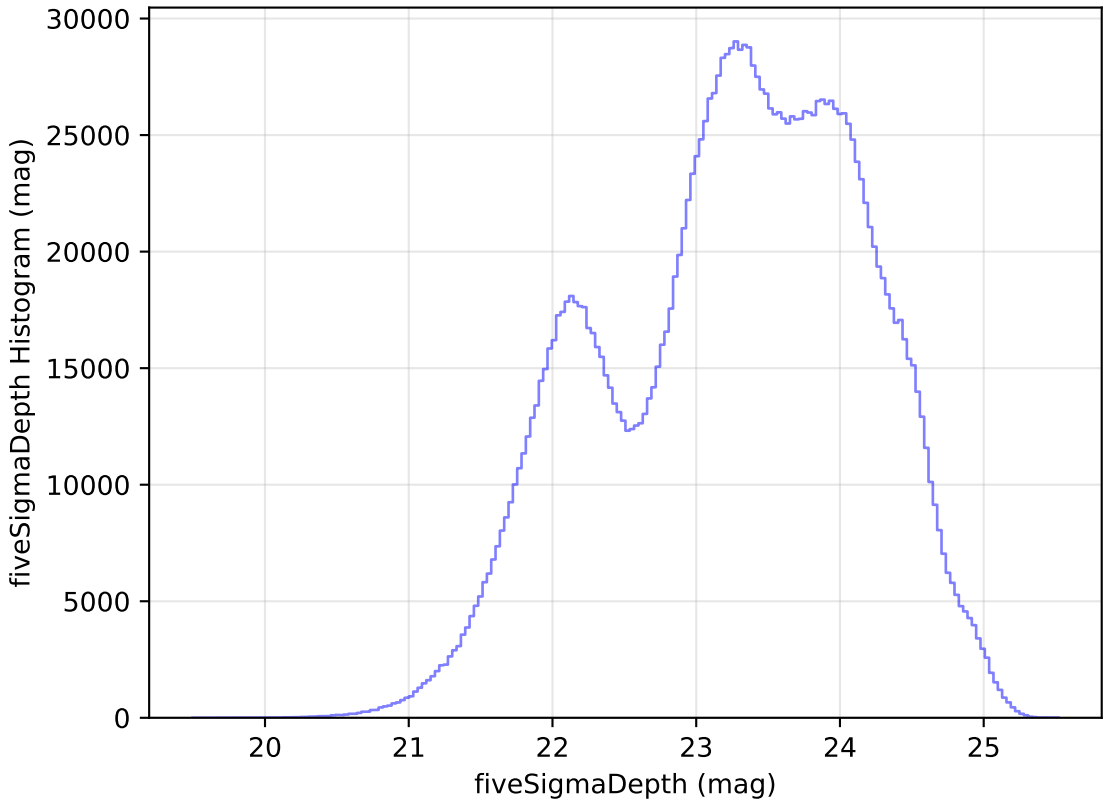
roman_v3.3_10yrs All sky all bands: fiveSigmaDepth Histogram
