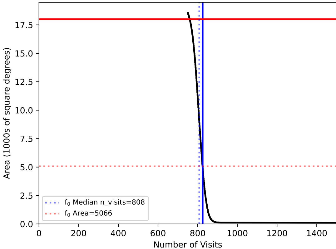
roman_v3.3_10yrs WFD: f0
