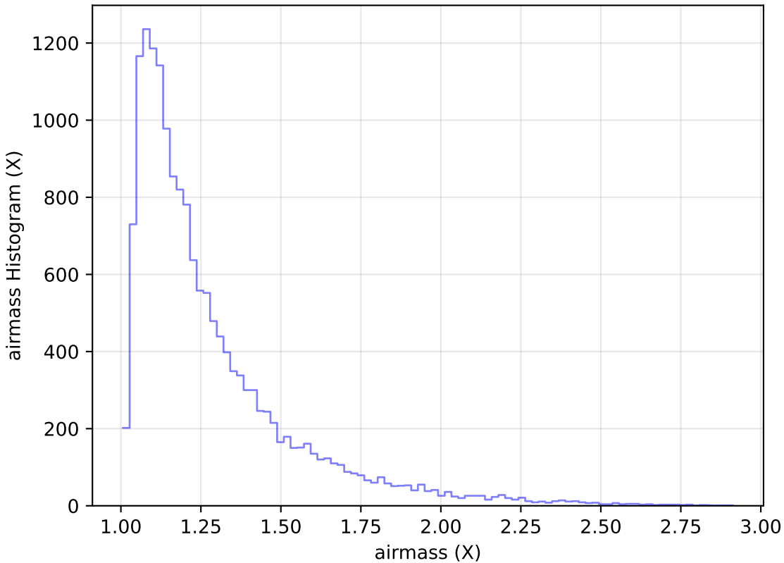
roman_v3.3_10yrs Yr 1 u band: airmass Histogram
