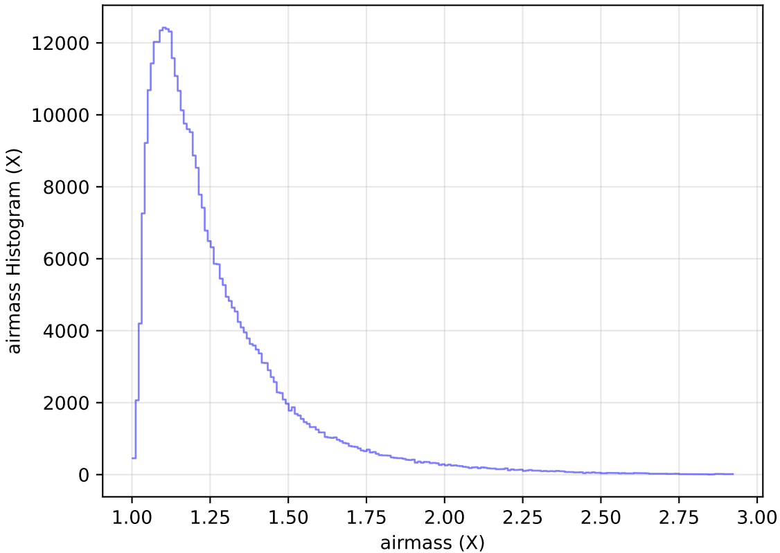
roman_v3.3_10yrs WFD y band: airmass Histogram
