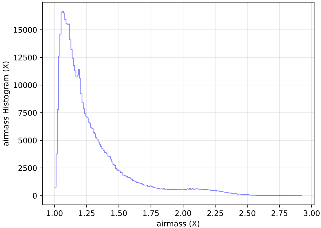
roman_v3.3_10yrs WFD r band: airmass Histogram
