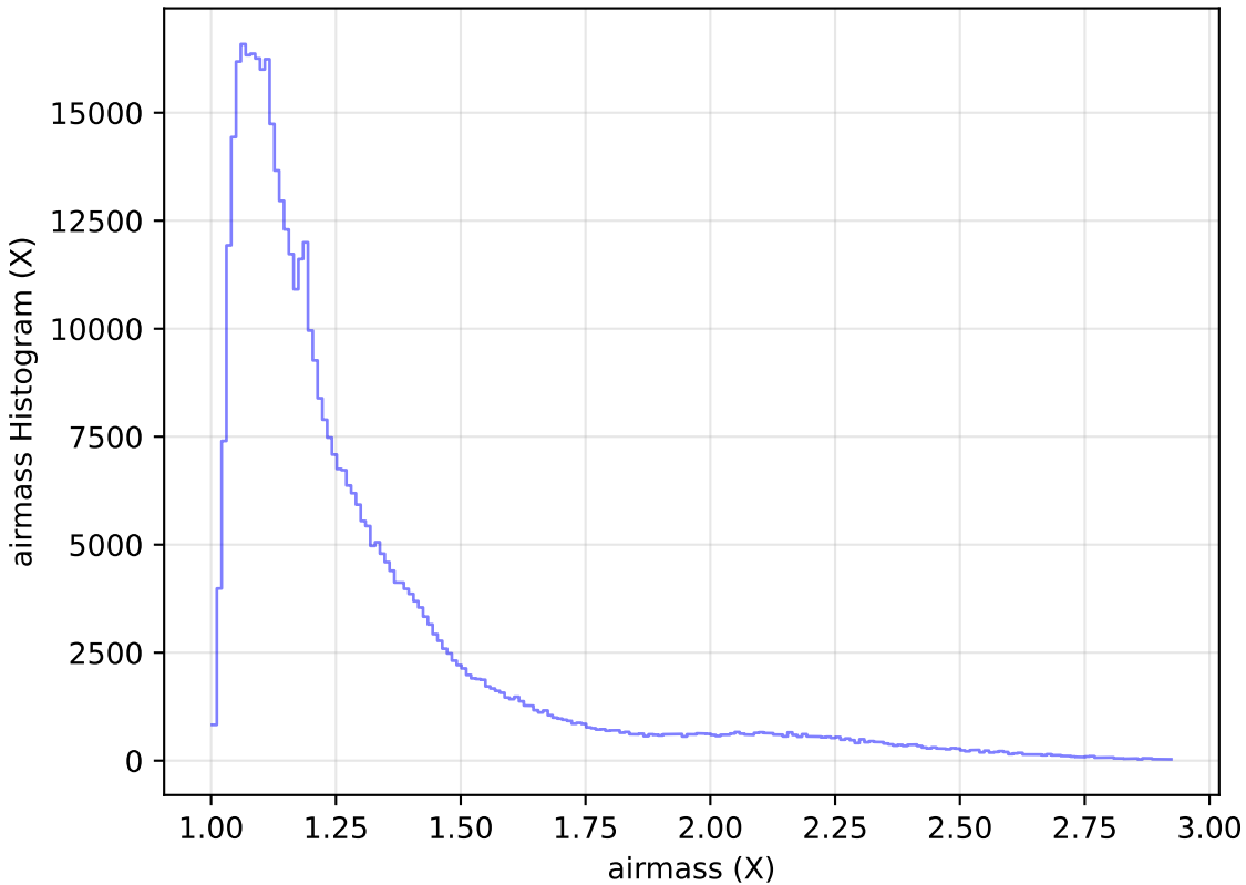
roman_v3.3_10yrs WFD i band: airmass Histogram
