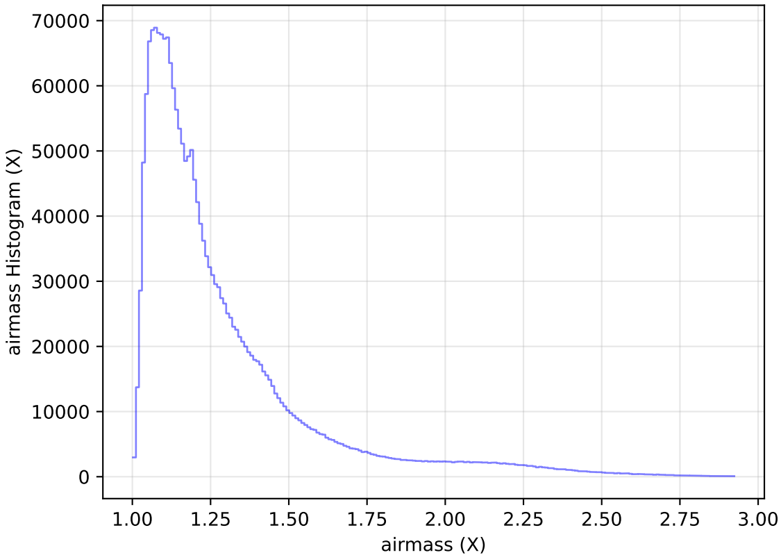
roman_v3.3_10yrs WFD all bands: airmass Histogram
