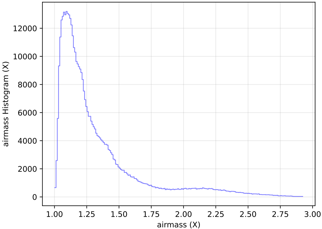
roman_v3.3_10yrs All sky z band: airmass Histogram
