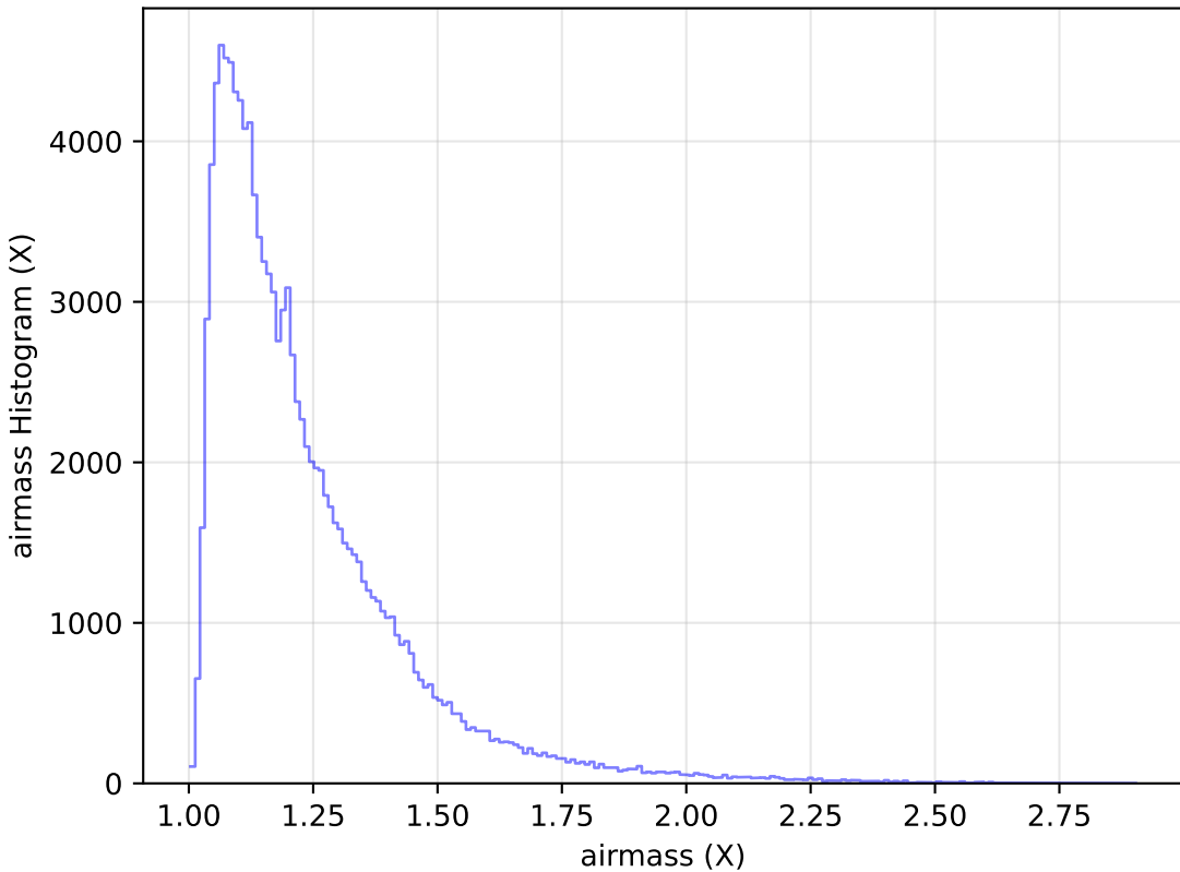
roman_v3.3_10yrs All sky u band: airmass Histogram
