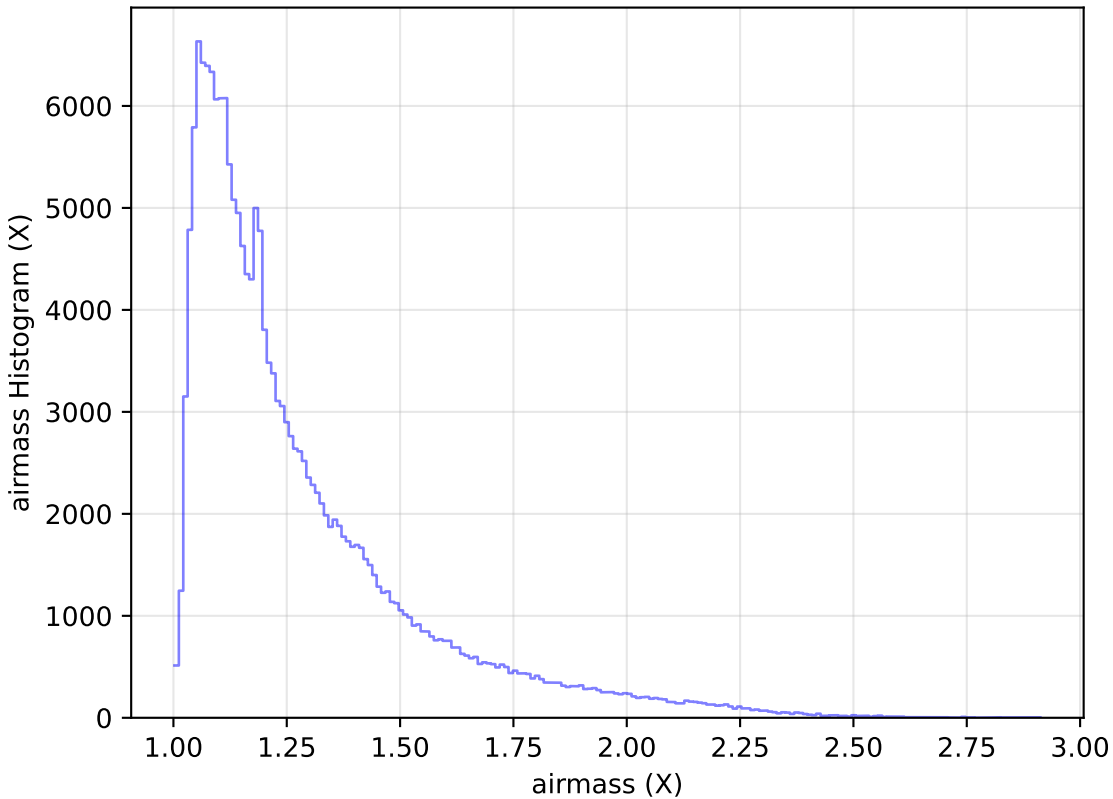
roman_v3.3_10yrs All sky g band: airmass Histogram
