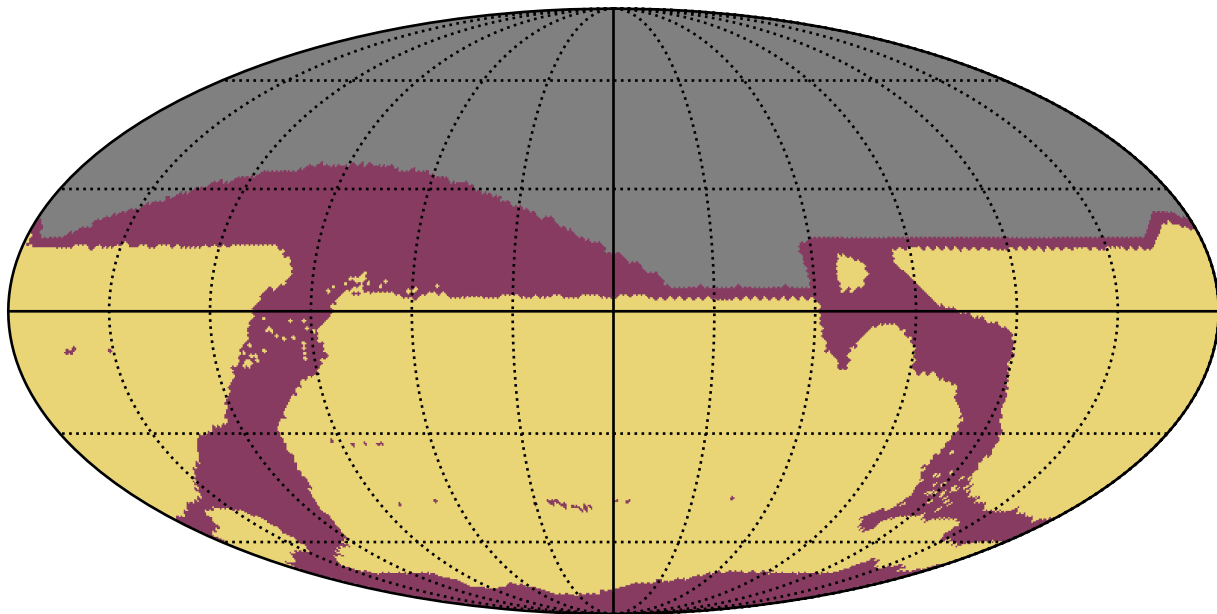
roman_v3.3_10yrs All sky: RapidRevisits
