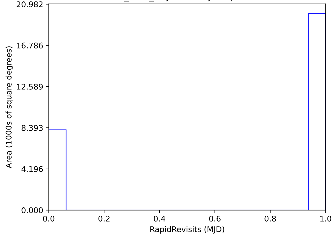
roman_v3.3_10yrs All sky: RapidRevisits
