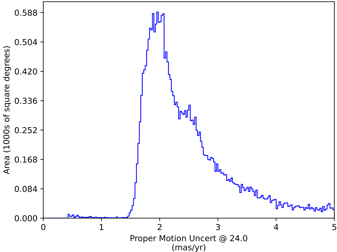
roman_v3.3_10yrs All sky: Proper Motion Uncert @ 24.0
