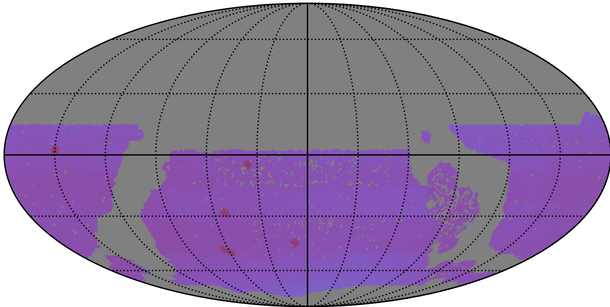
roman_v3.3_10yrs WFD: Proper Motion Uncert @ 20.5
