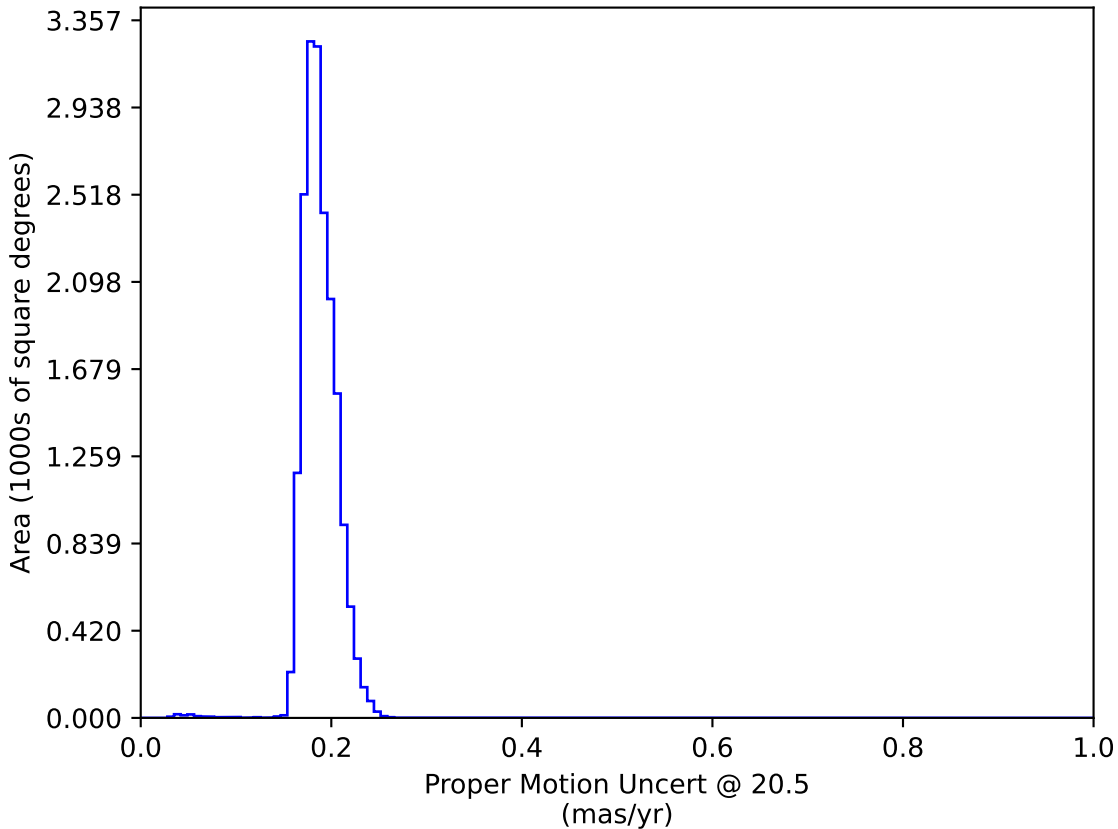
roman_v3.3_10yrs WFD: Proper Motion Uncert @ 20.5
