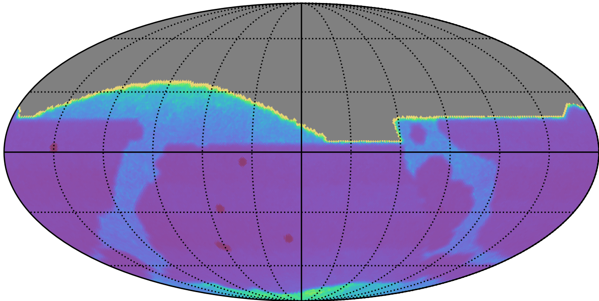
roman_v3.3_10yrs All sky: Proper Motion Uncert @ 20.5
