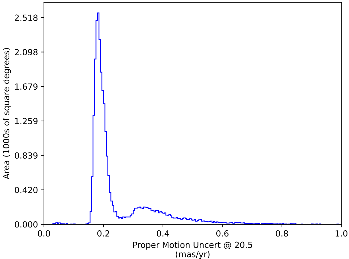
roman_v3.3_10yrs All sky: Proper Motion Uncert @ 20.5
