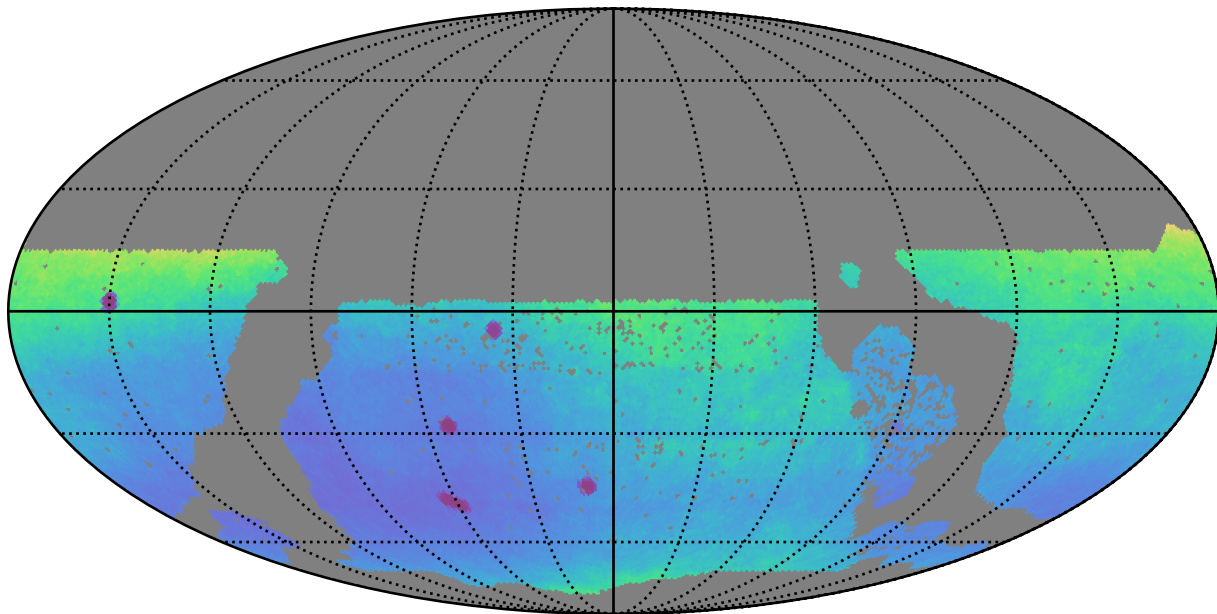
roman_v3.3_10yrs WFD: Parallax Uncert @ 24.0
